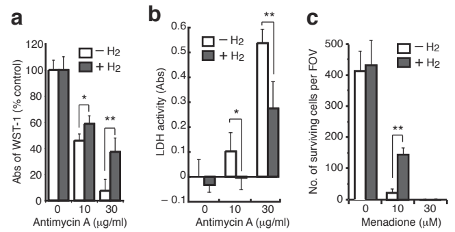
Supplementary Figure 3 Several methods confirm protection of cells by \text{H}_2 against oxidative stress.
